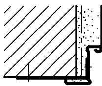
Dübelmontage Variation 1
