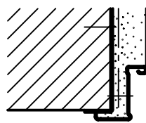
Dübelmontage Variation 2
